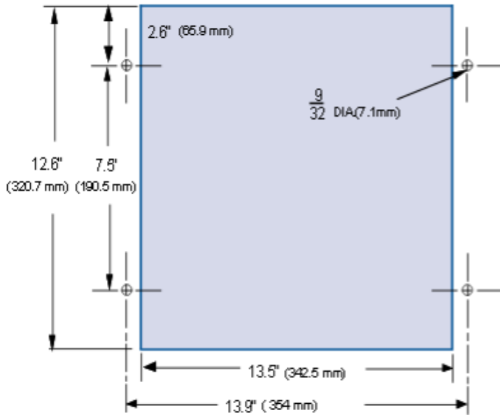
Panel cut-out for flush mounting
