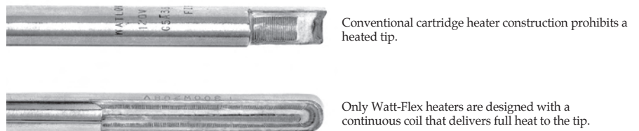
Figure 5: Watt-Flex Hot Tip Heater vs. Conventional Heater
