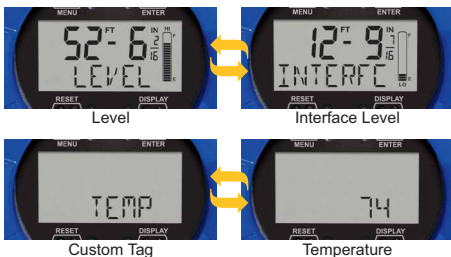
display interface level & temperature
